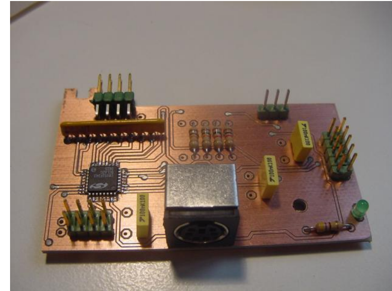
PS/2 keyboard adapter, 2006
